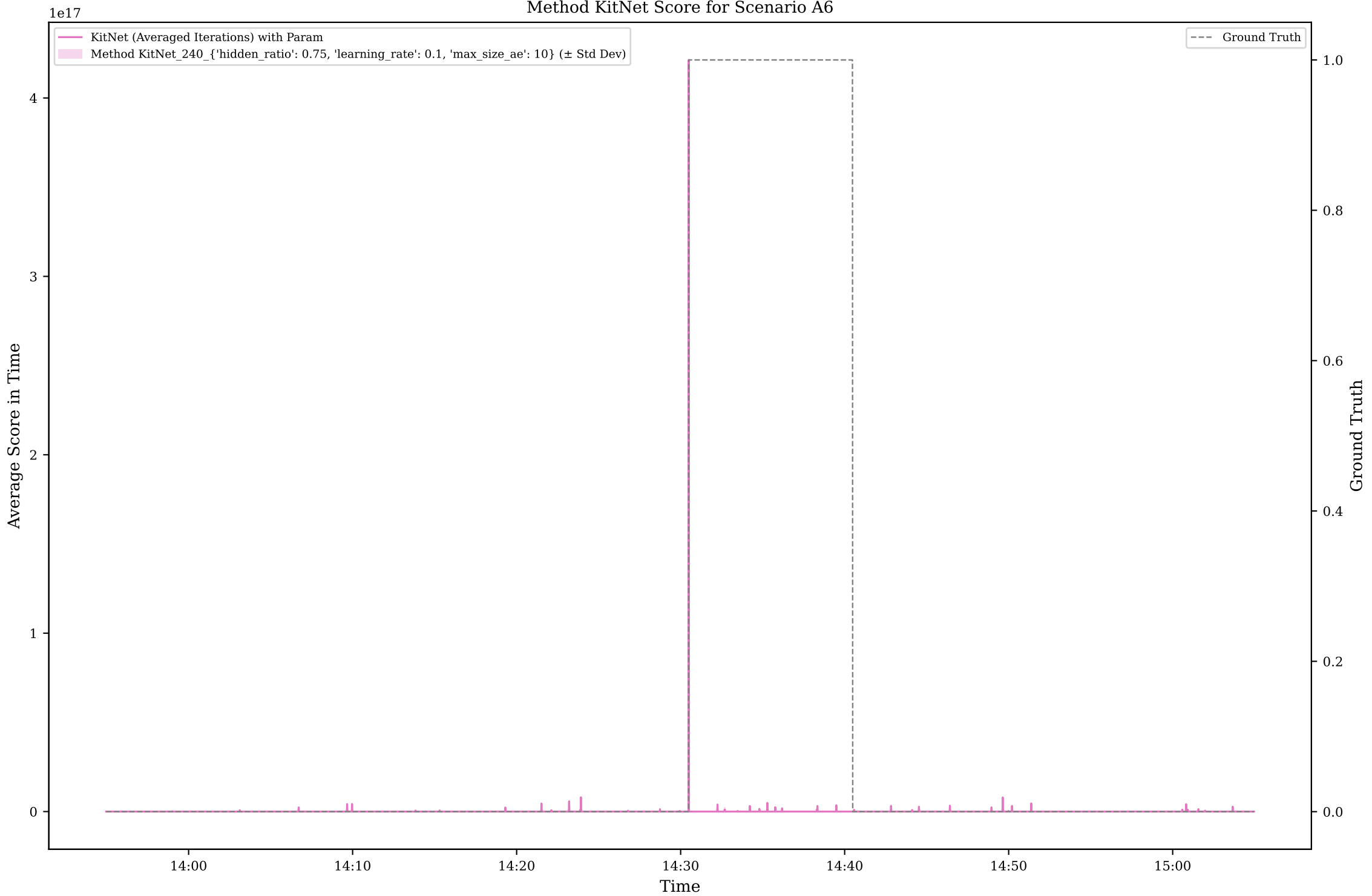
Method KitNet Score for Scenario A6
